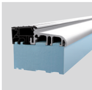
THRESHOLD FOAM BOARD 23 5⁄8 in x 11 7⁄8 in x 43 3⁄8 in
